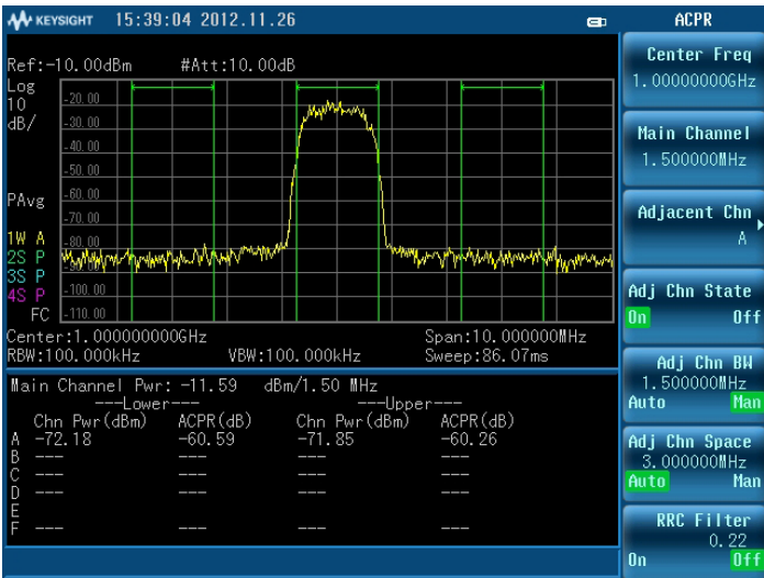
Figure 2. ACPR measurement
