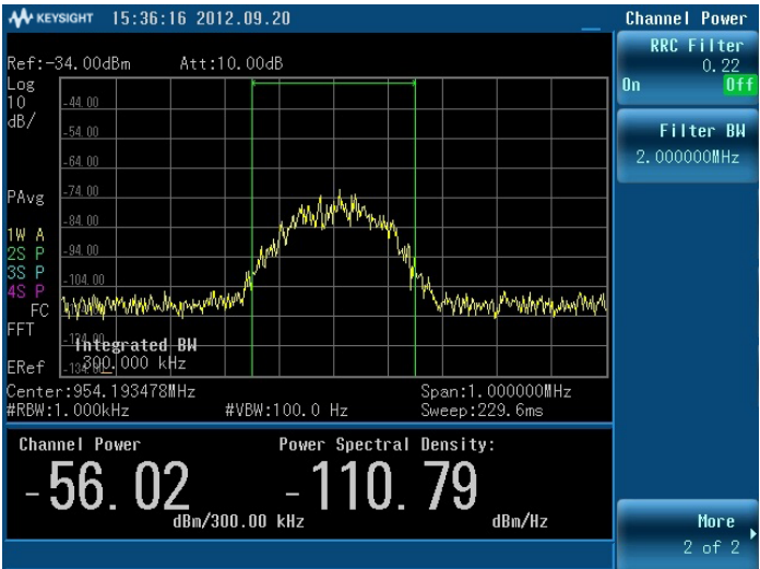
Figure 1. Channel power measurement
