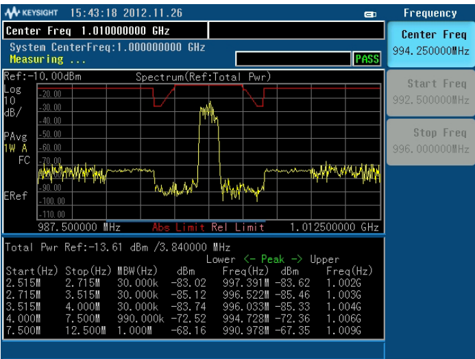
Figure 3. SEM measurement
